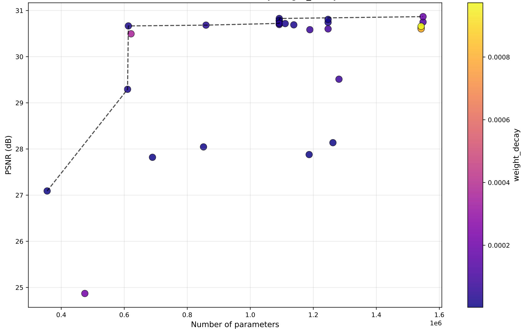
PSNR vs #Params — HAT — by weight_decay
